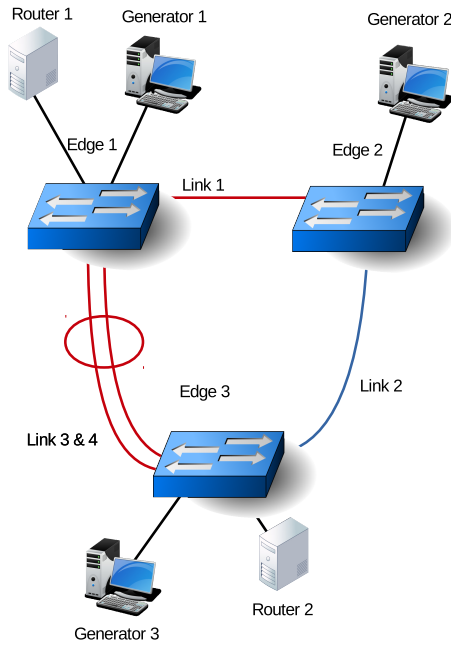
Figure 3. TouSIX test topology
