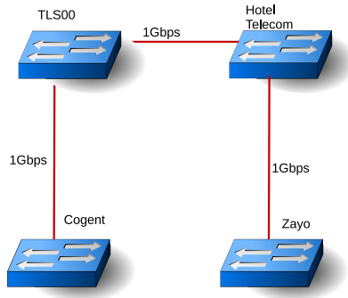
Figure 1. TouIX legacy architecture
