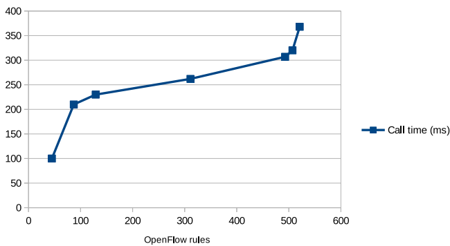
Figure 7. Rules Generation module execution time
